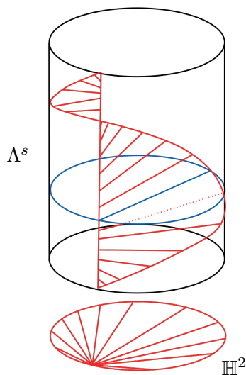
FIGURE 3. A picture of \tilde{\sigma}(\tilde{M}) in the familiar case M = \text{UT}\Sigma as in [47]. The infinite cylinder is \tilde{\sigma}(\tilde{M}) \cong \tilde{M} = \mathbb{H}^2 \times \Lambda^s i.e. the height of a point in the stack of copies of \mathbb{H}^2 corresponds to the positive endpoint of a unit tangent vector based at that point. Horizontal planes are leaves of \mathcal{F}^s , one is shown in blue. A leaf of \tilde{\sigma}(\mathcal{F}^u) is shown in red, the hyperbolic metric on the leaf is that lifted from the projective model of \mathbb{H}^2 shown below. In this model, one endpoint at infinity of the unstable leaf is blown up to an interval.
