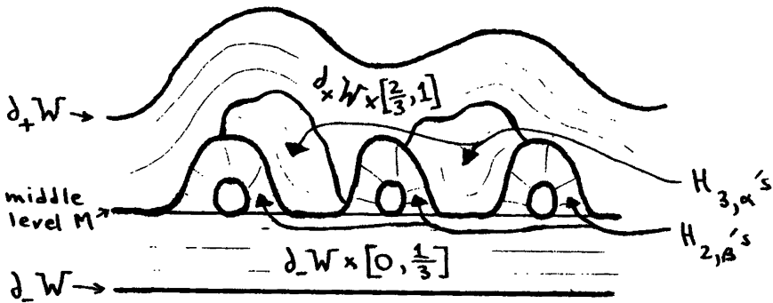
Figure 8.2: The cobordism W .
