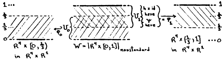
Figure 8.1: Defining W
