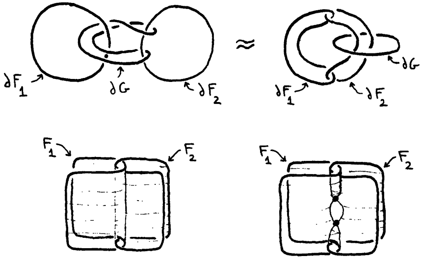
Before finger move; F_1 \cap F_2 = \emptyset After finger move; F_1 \cap F_2 = 2 points
