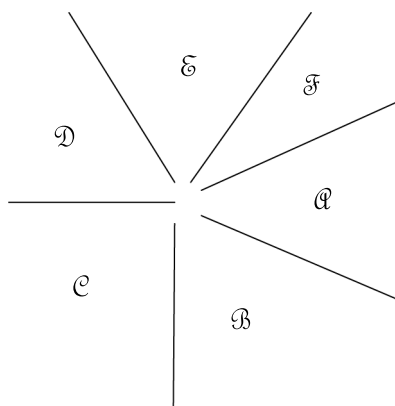
Fig. 10 Very high-level overview of how the plane is partitioned into regions.
