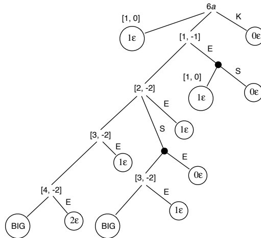
Fig. 7 Game tree of Figure 6a.
