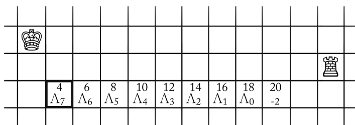
Fig. 17 Some values in \mathcal{D}+ .
