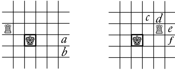
Fig. 6 Some positions of value \{1\epsilon|\epsilon\} in Echess.
