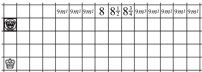
Fig. 20 Some values in column x = 0 of \mathcal{C}' .
