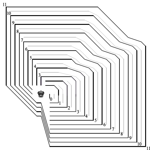
Fig. 3 Contours of the mean value with Black king at [0, 0] ; rook at [-2, 1] .
