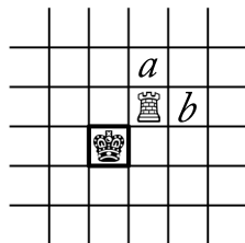
Fig. 4 Two "terminal" positions in Echess.
