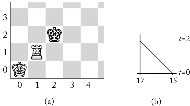
Fig. 1 Initial configuration in the “King and Rook vs. King on a quarter-infinite board” problem and thermograph.
