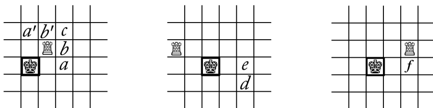
Fig. 5 More positions of value \varepsilon . We define e' , d' and f' by reflecting both the White king and rook across the diagonal through the Black king.
