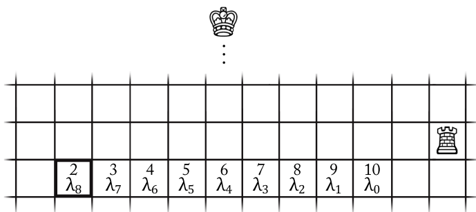
Fig. 16 Some values of the opening sequence in \mathfrak{E}_{wN} .
