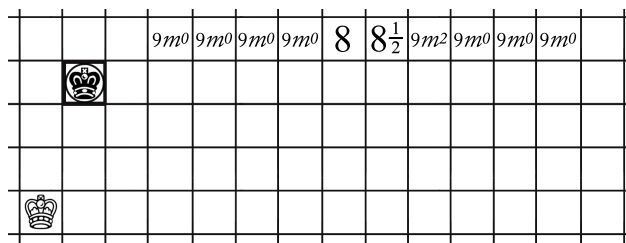
Fig. 19 Some values in column x = -1 of \mathcal{C}' .
