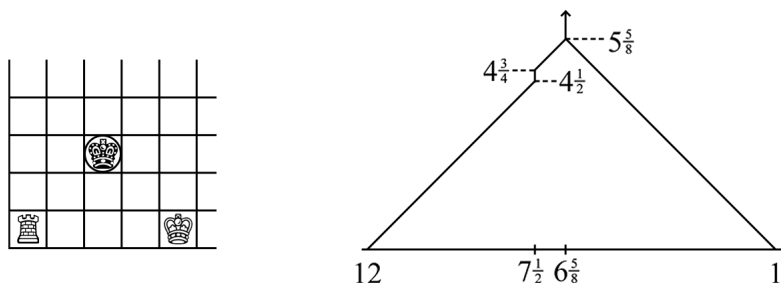
Fig. 27 An Eches position with temperature 5\frac{5}{8} .
