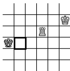
Fig. 9 A “near-terminal” position which chills to \frac{1}{2} .
