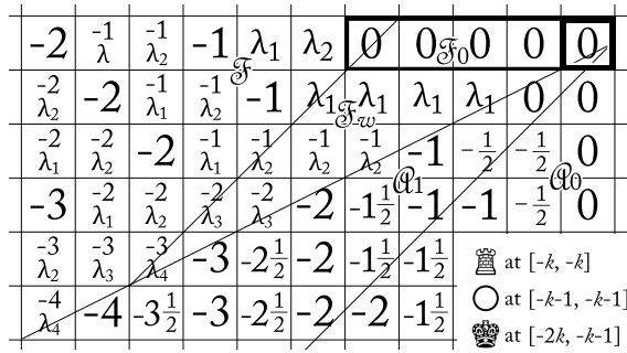
Fig. 23 values in \mathfrak{F}_0 and \mathfrak{F}_w .
